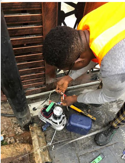
Gate Automation Machine Installation
